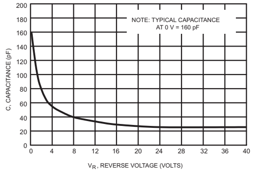
FIG. 6- TYPICAL CAPACITANCE
